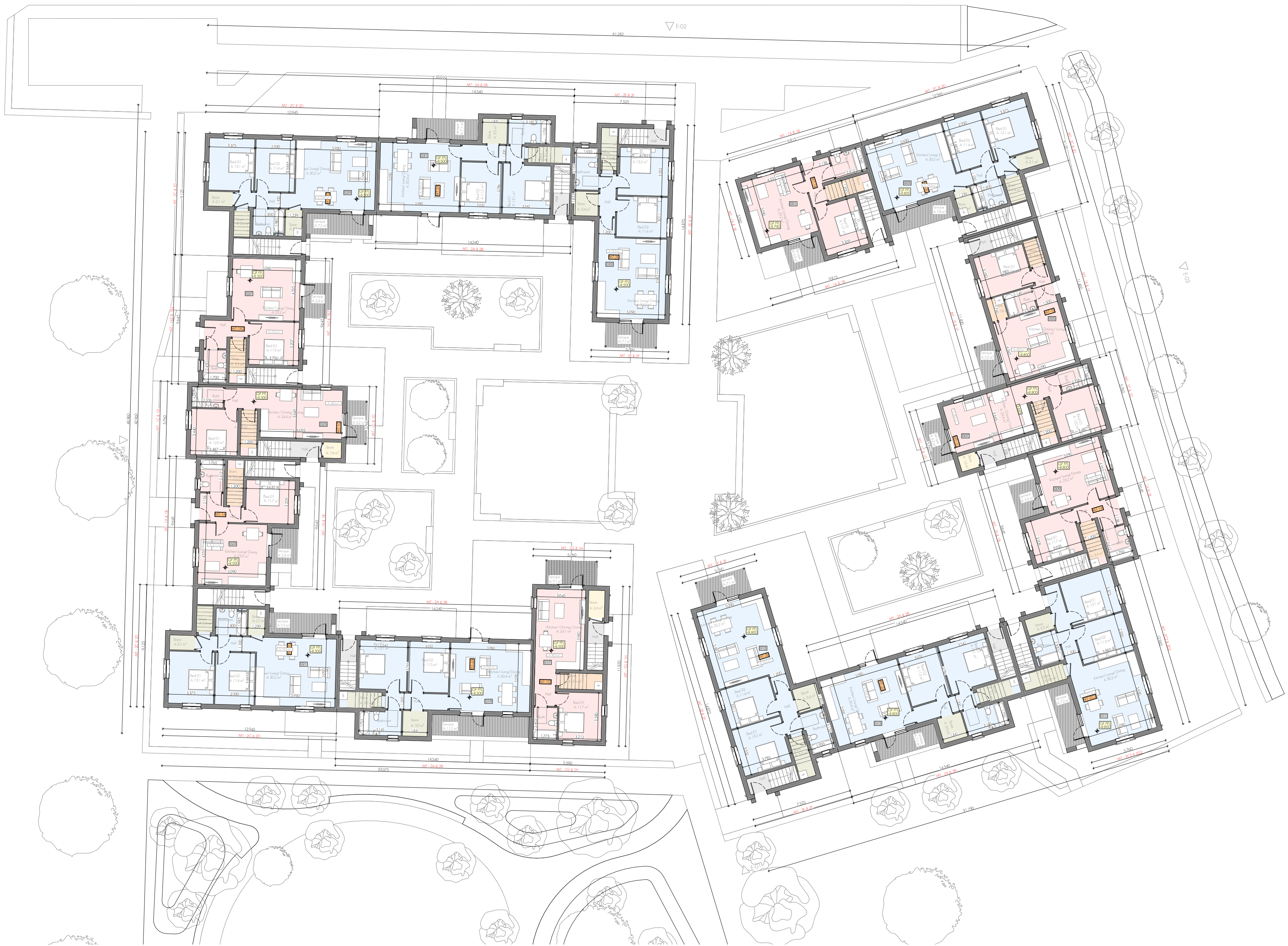
Proposed Ground Floor Plan 1:200
