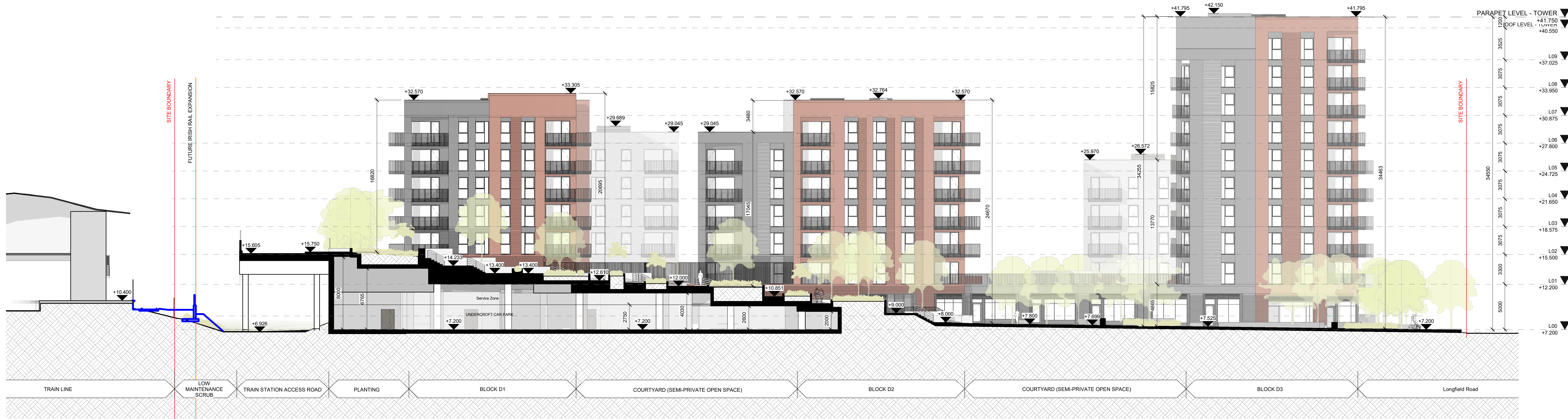
2 STAPOLIN SQUARE - EAST WEST SECTION 02 1 : 200
