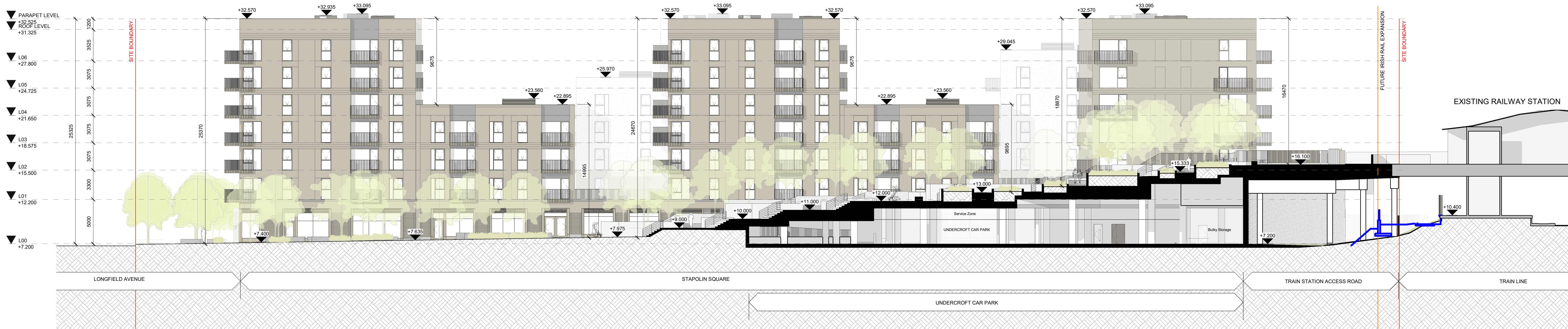
1 STAPOLIN SQUARE - EAST WEST SECTION 01 1 : 200
