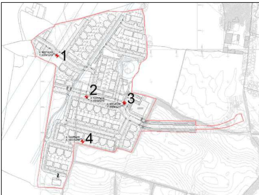
Figure 2: Site Infiltration Test Locations
