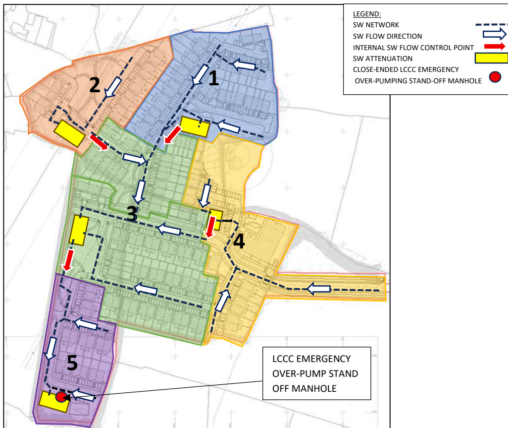
Figure 3: Surface Water Sub-Catchments
