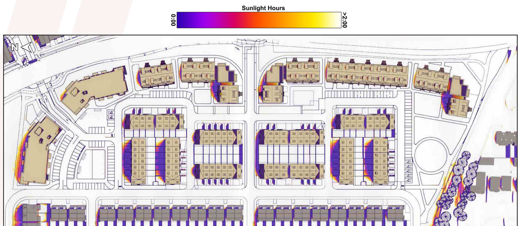
Figure C.32: Area capable of receiving 2 hours of sunlight on March 21st shown in white
