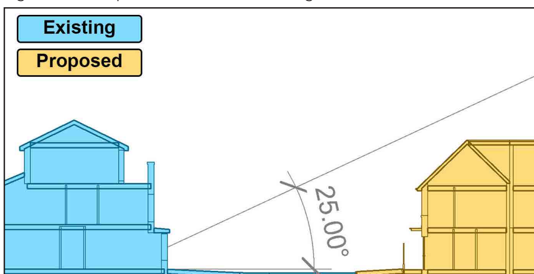
Figure 2.4: Example Section B-B taken through Phase 1 unit 28
