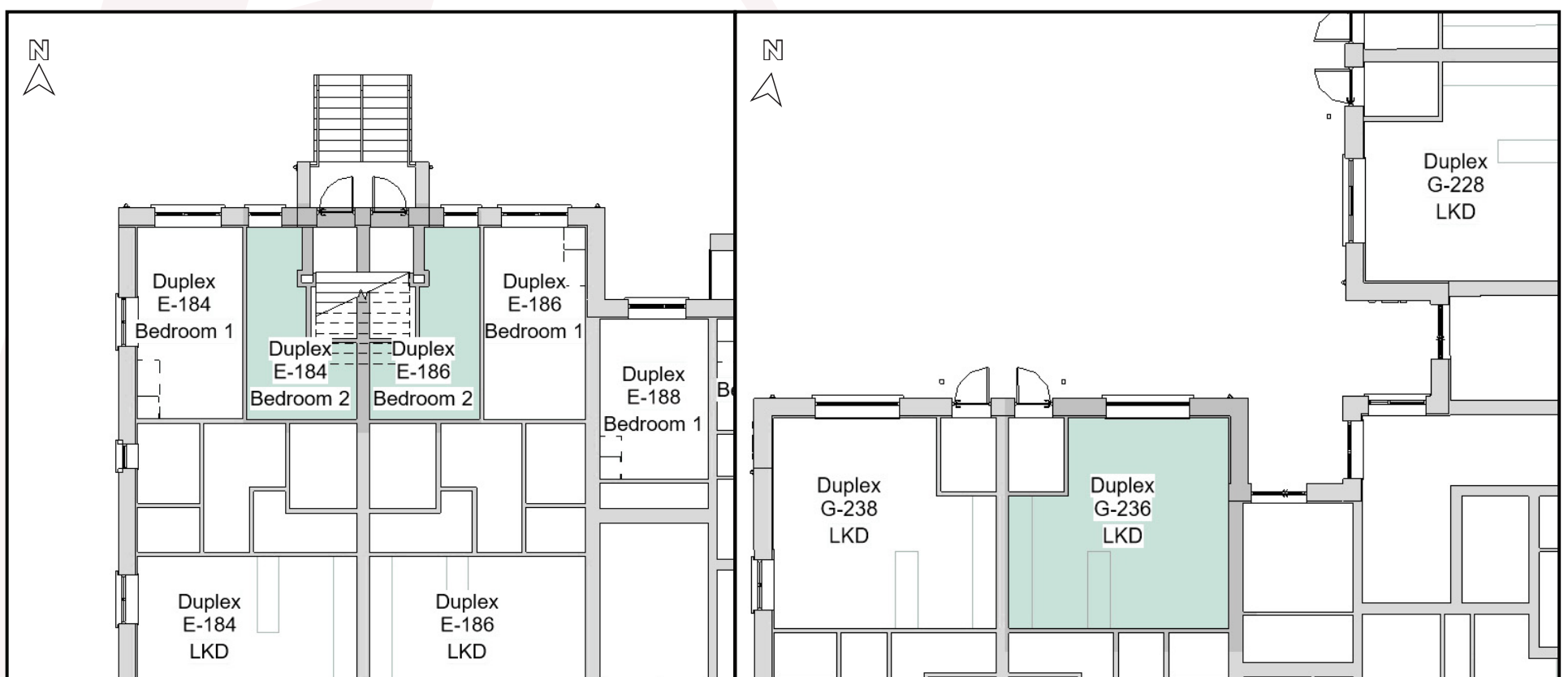
Figure 3.3: Duplex Block E Ground Floor Plan (L), Duplex Block G, Ground Floor Plan (R)
