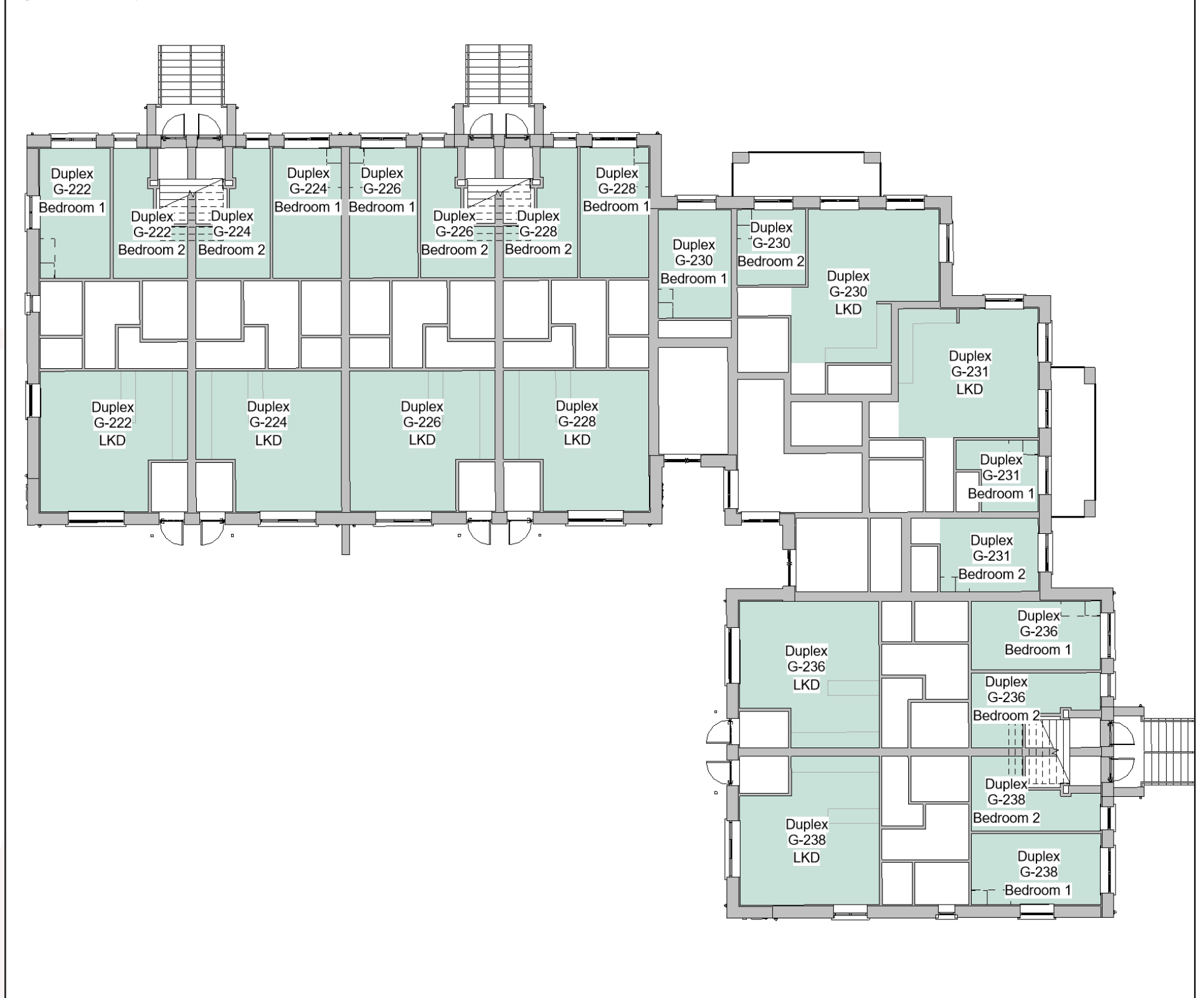
Figure C.28: Duplex Block G - Ground Floor
