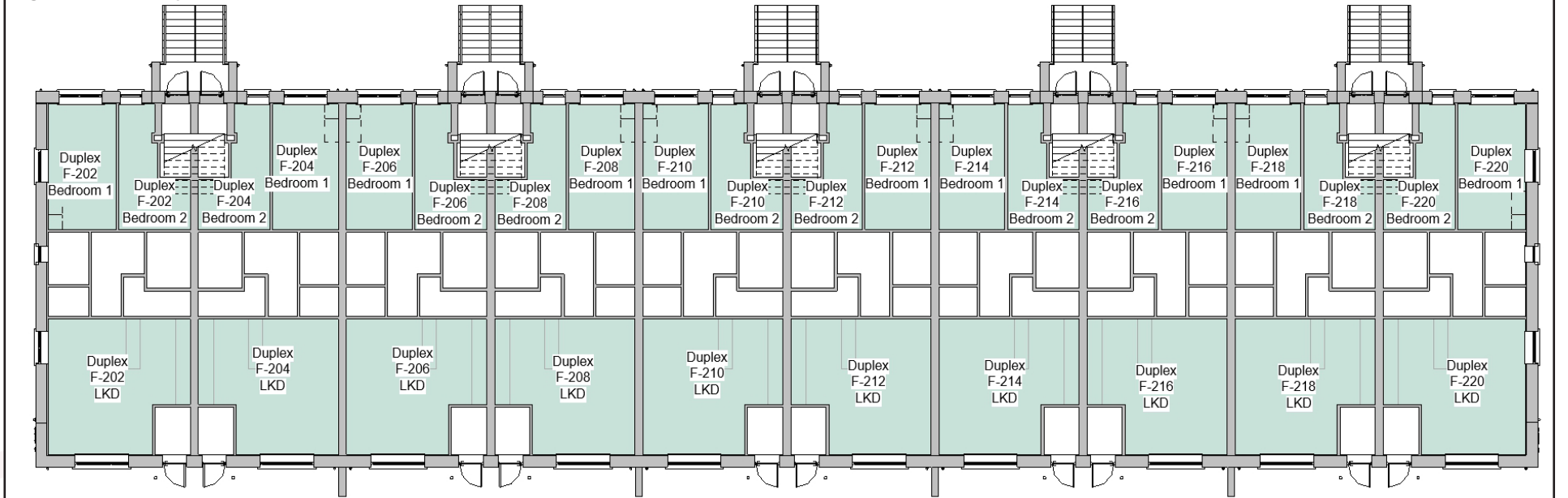
Figure C.25: Duplex Block F - First Floor
