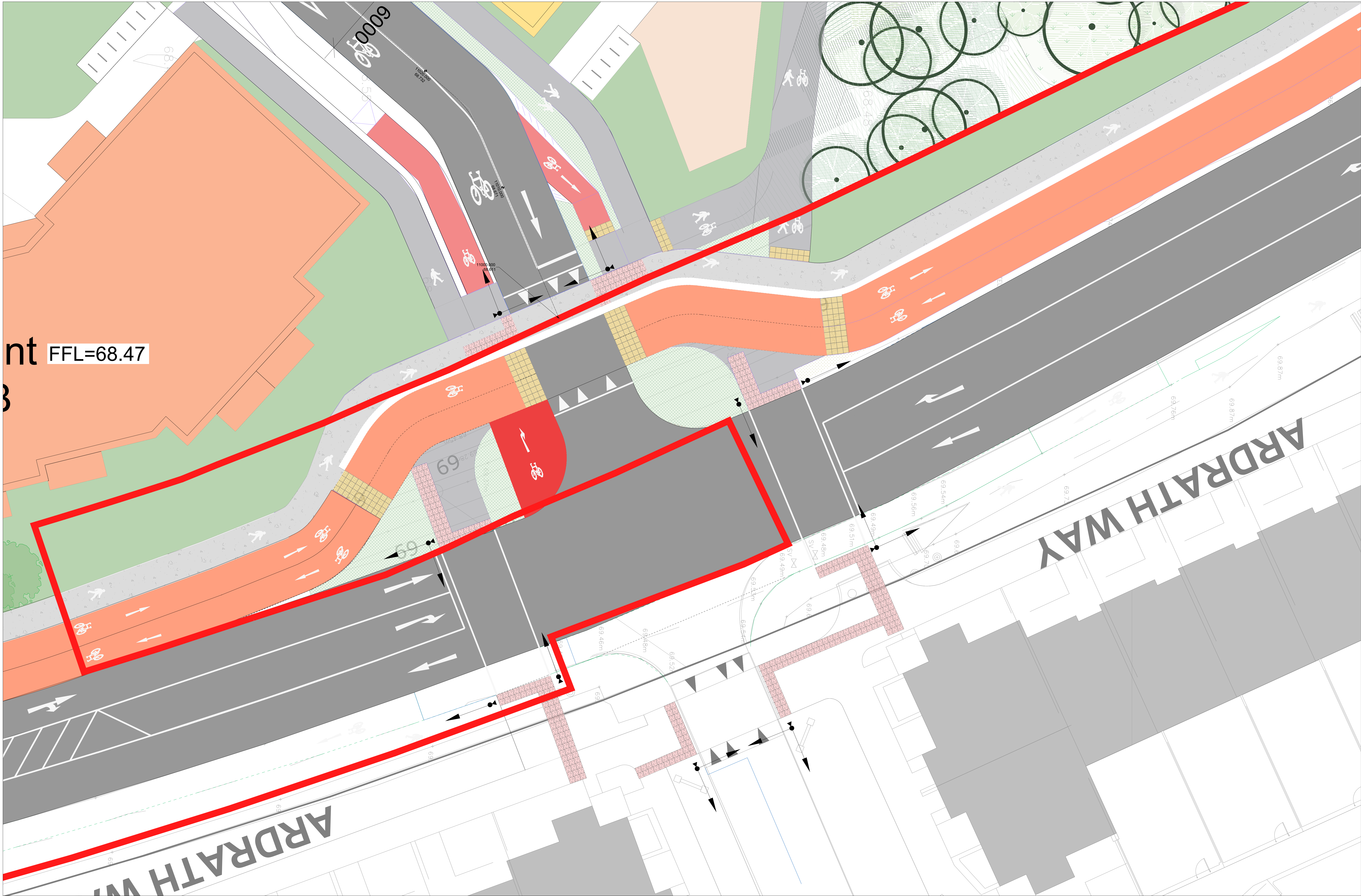
DETAIL FOR JUNCTION 3 SCALE @ A2: 1:100 SCALE @ A3: 1:200
