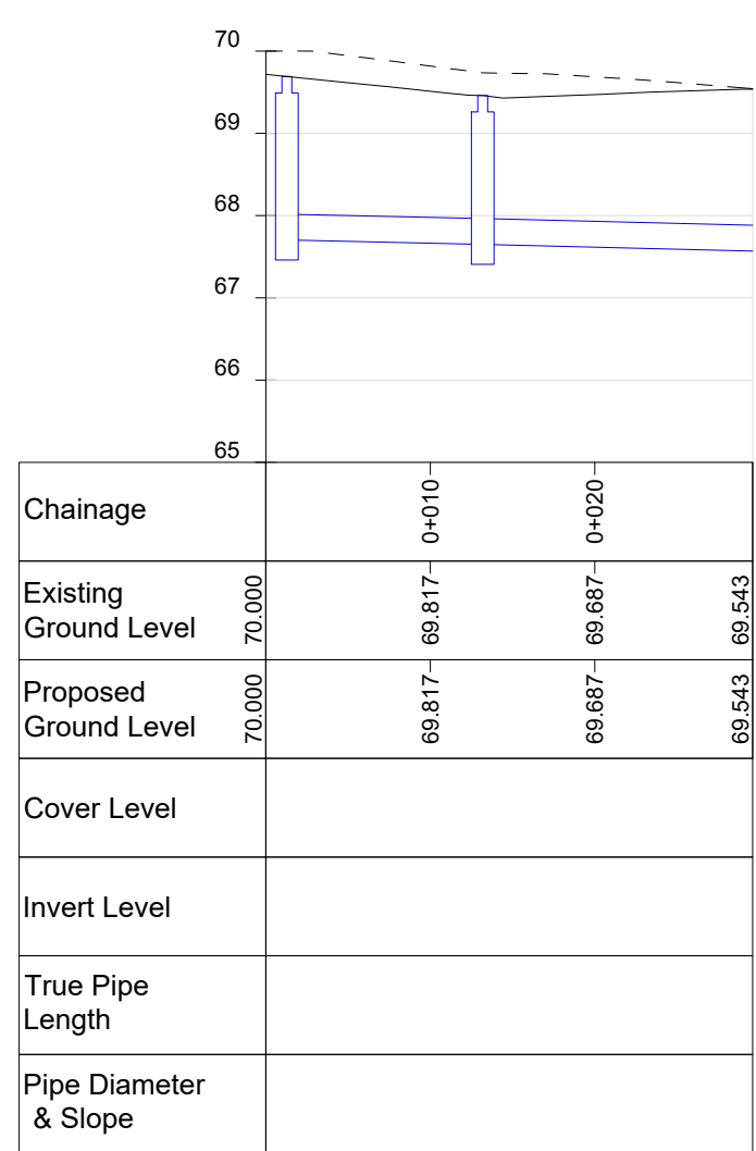
SECTION S11.4 TO S11.5 H=1:500,V=1:100
