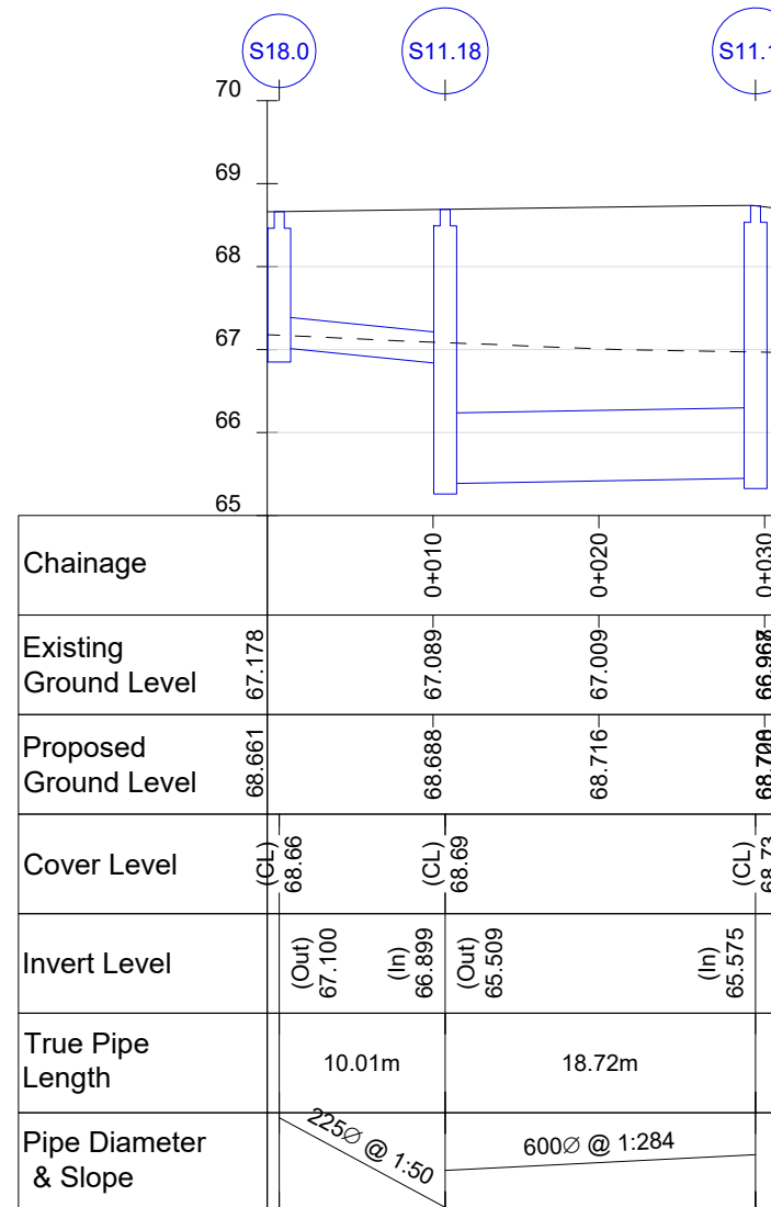
SECTION S18 TO S11.17 H=1:500,V=1:100
