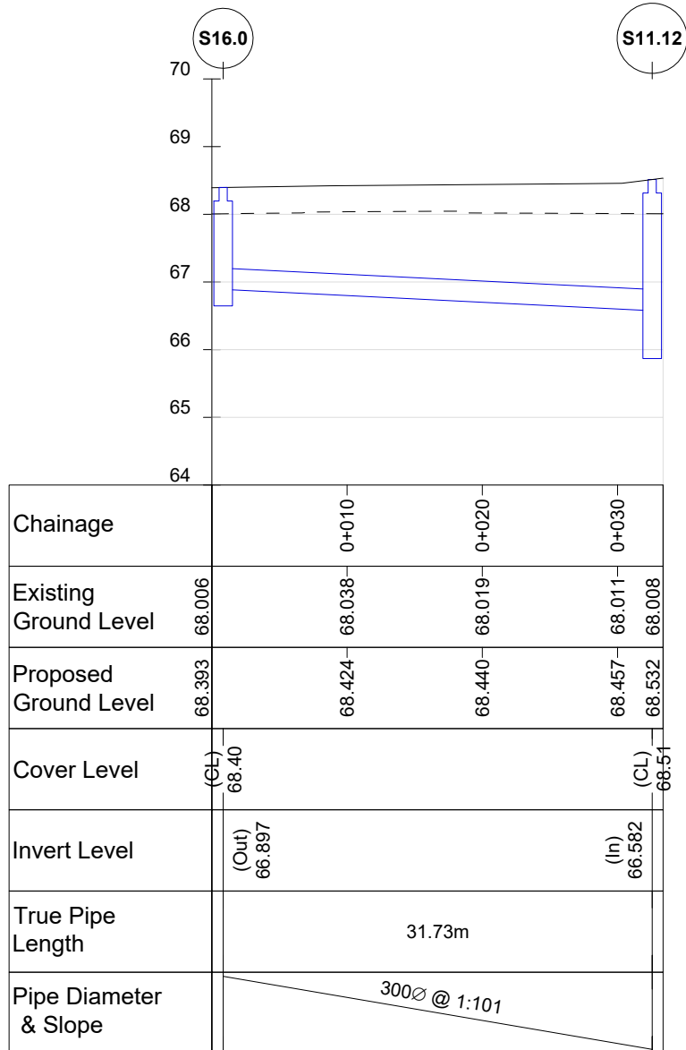
SECTION S11.14 TO S16.0 H=1:500,V=1:100
