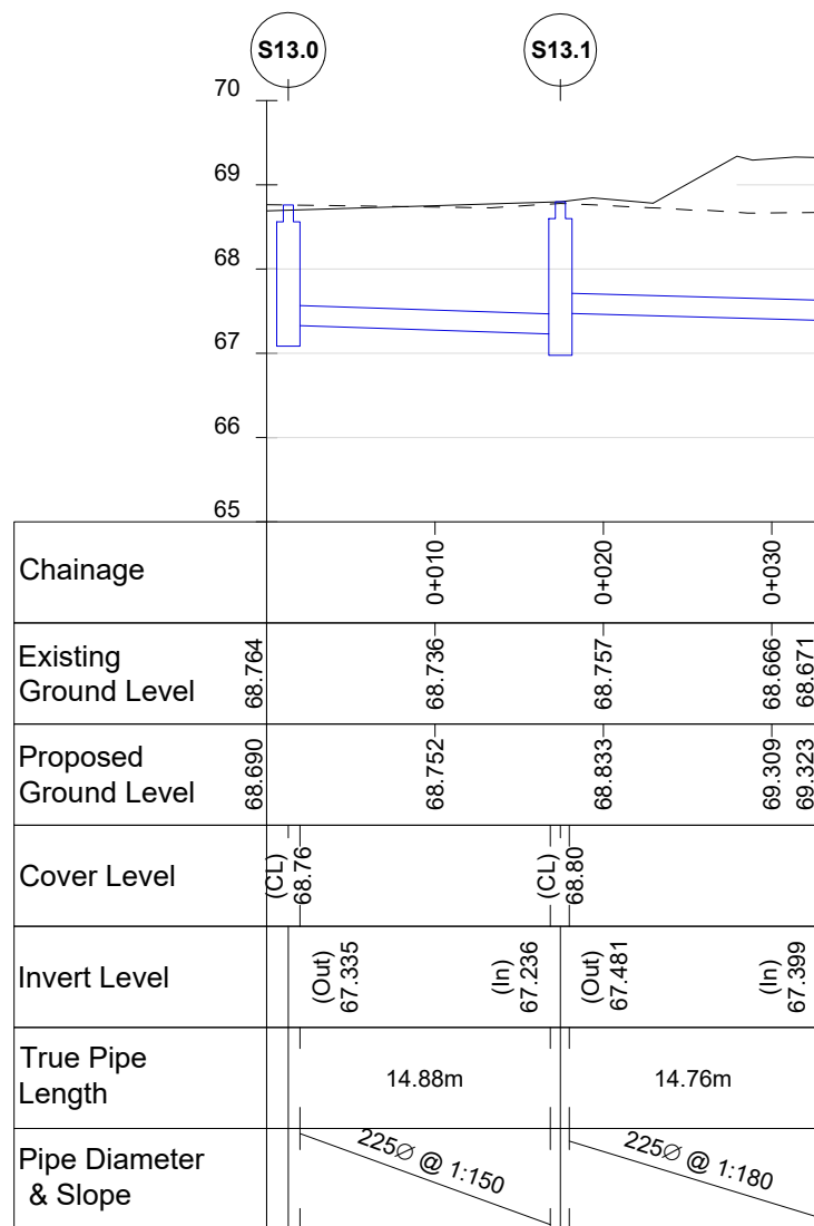
SECTION S13 TO S13.1 H=1:500,V=1:100
