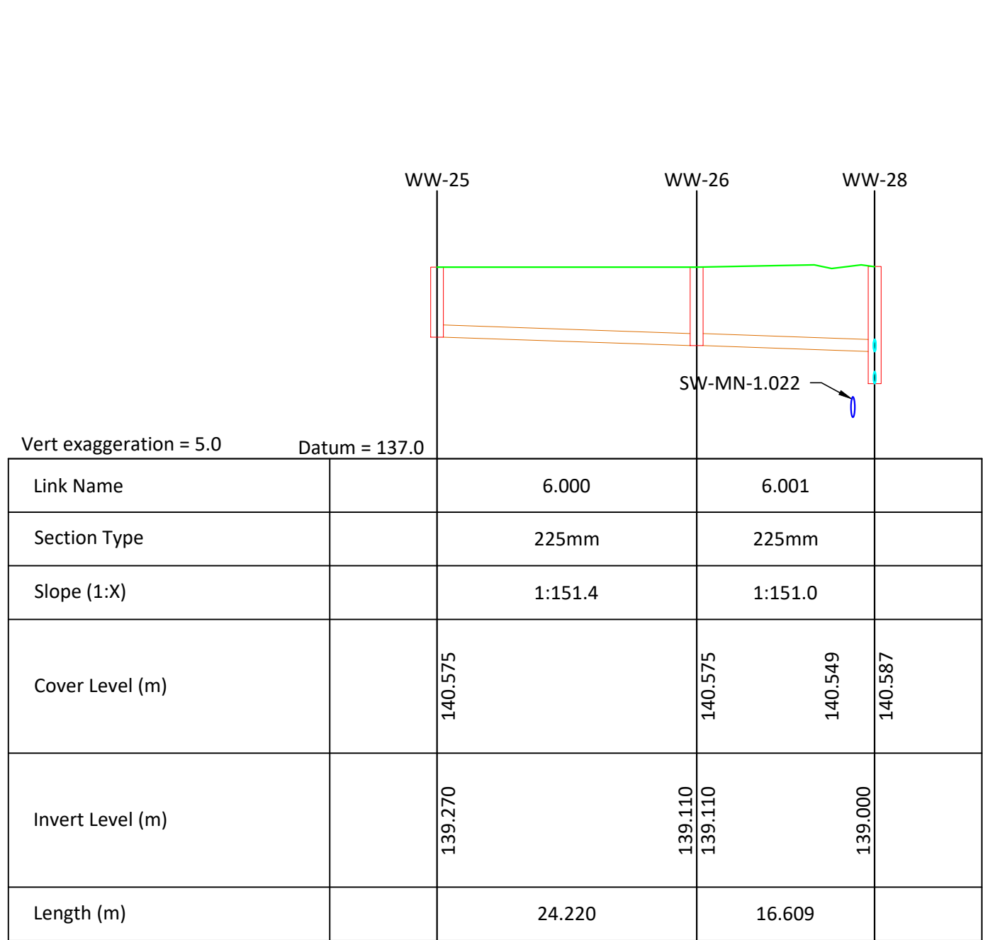
SURFACE WATER NETWORK WW-6.000 - WW-6.001
