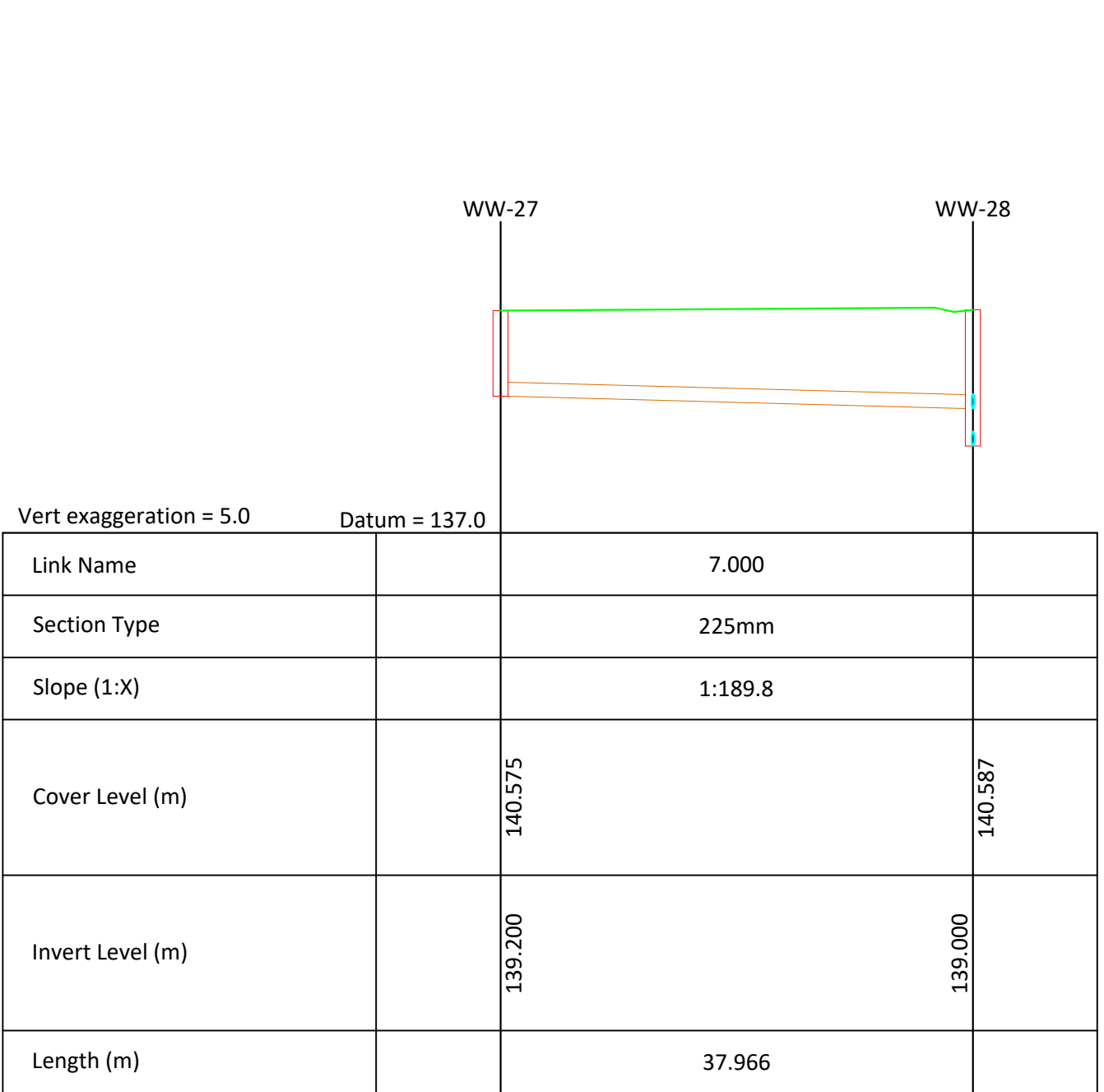
SURFACE WATER NETWORK WW-7.000
