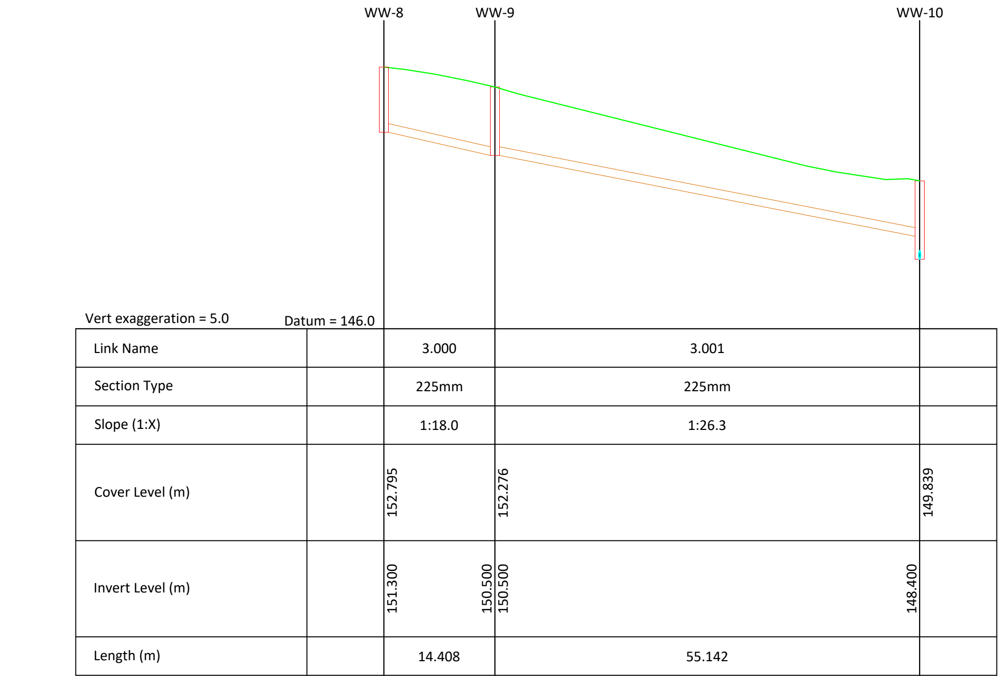
SURFACE WATER NETWORK WW-3.000 - WW-3.001
