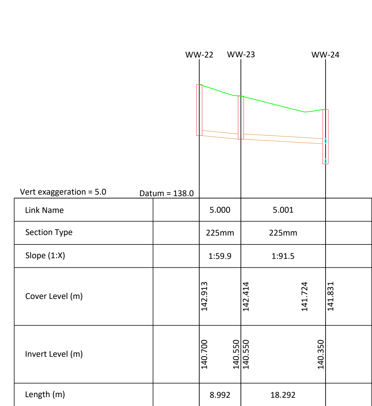
SURFACE WATER NETWORK WW-5.000 - WW-5.001
