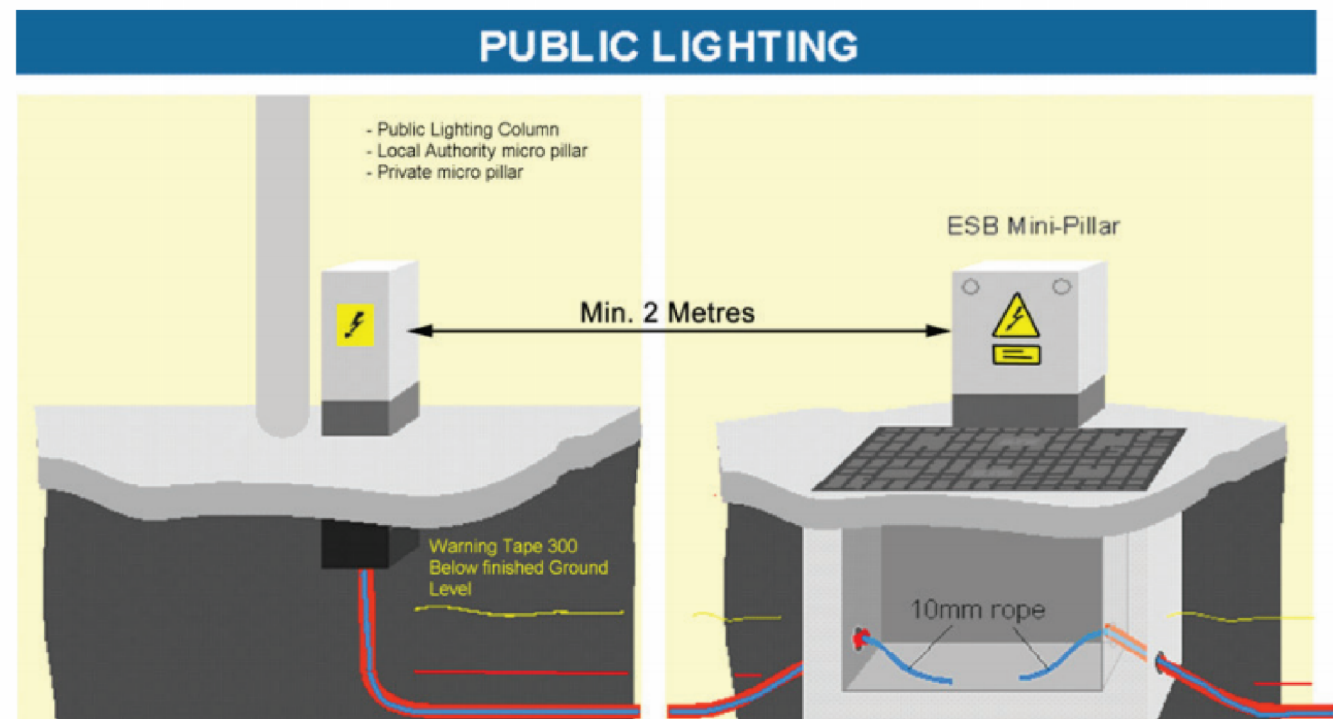
DETAIL No.1 ESB STANDARD FOR MICRO PILLARS SCALE N.T.S.
