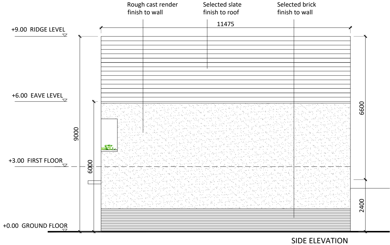
SIDE ELEVATION
