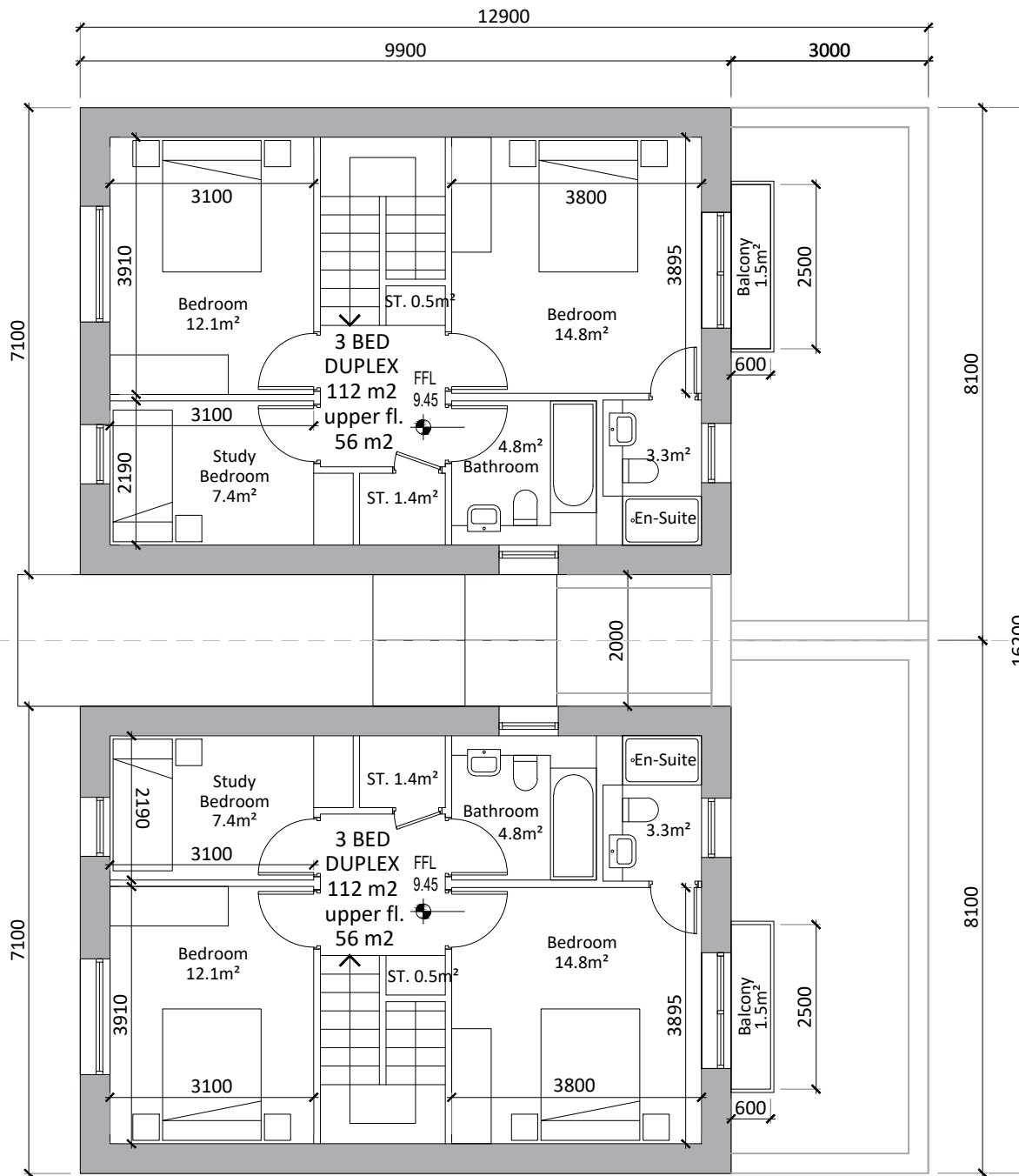
BLOCKS C1 (DUPLEXES) _ PLAN LEVEL 03
