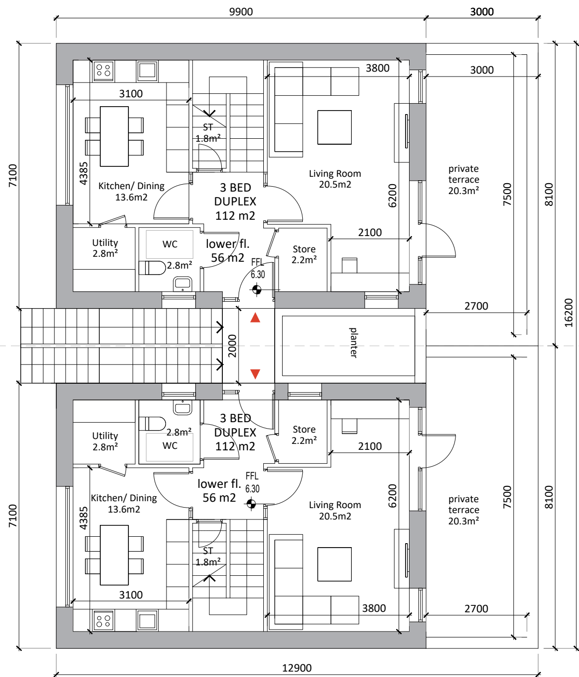
BLOCKS C1 (DUPLEXES) _ PLAN LEVEL 02
