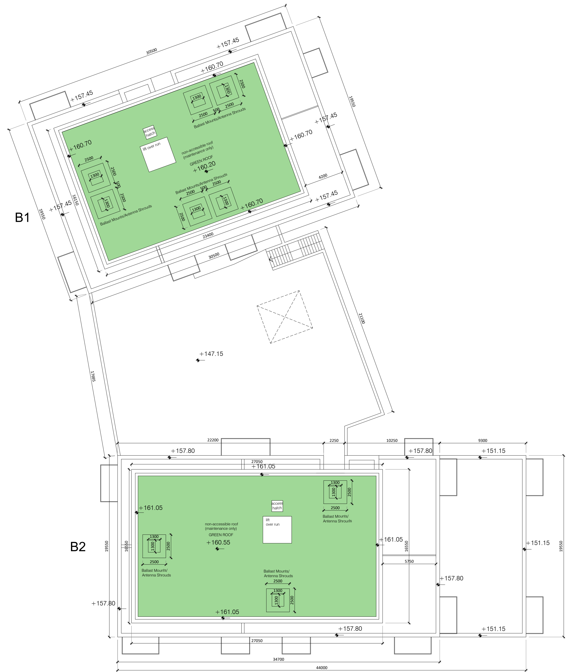
BLOCKS B1 + B2 _ PLAN LEVEL 05 _ ROOF LEVEL
